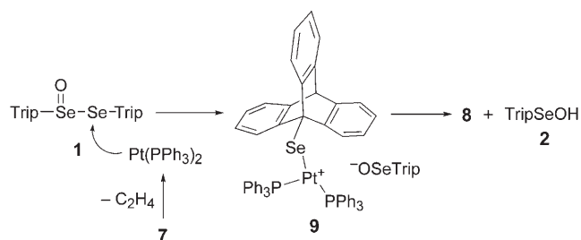
Scheme 2. A plausible mechanism for the reaction of selenoseleninate 1 with [\text{Pt}(\text{PPh}_3)_2(\eta^2\text{-C}_2\text{H}_4)] ( 7 ) to give selenaplatinacycle 8 .
